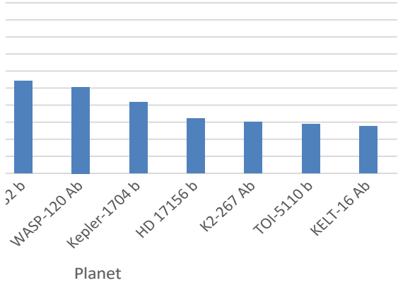
0 Planets by Mass
